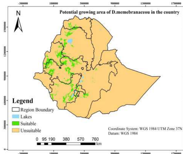
Fig 6. Suitable areas of D. membranaceus in different areas of Oromia, Amhara, Benishangul-Gumuz, SNNP, Tigray regions in Ethiopia
